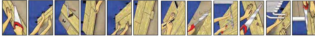
Picture 1: Before installing the first row, the part of the groove profile which sticks out must be cut off.
